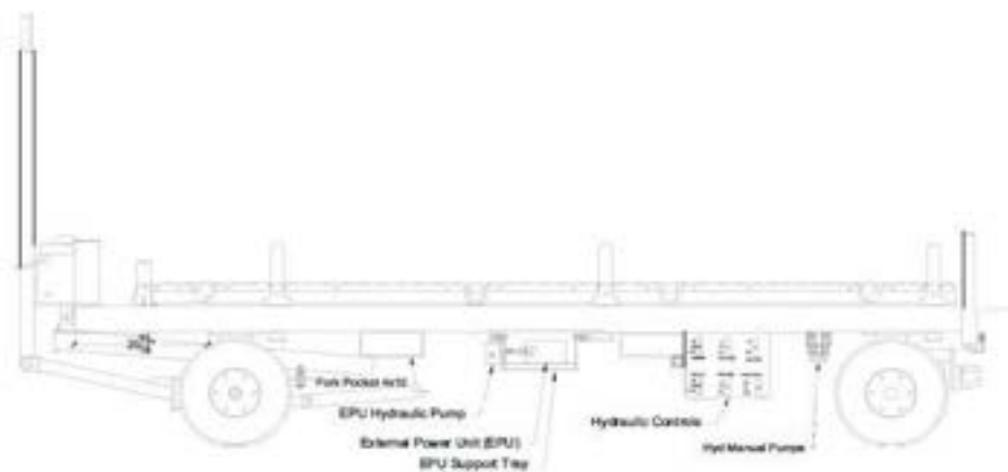
Side Elevation
