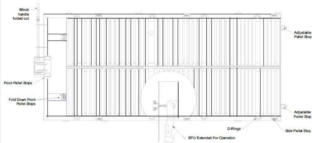
Top Elevation: EPU Extended For Operation
