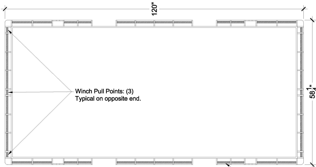
Top View
